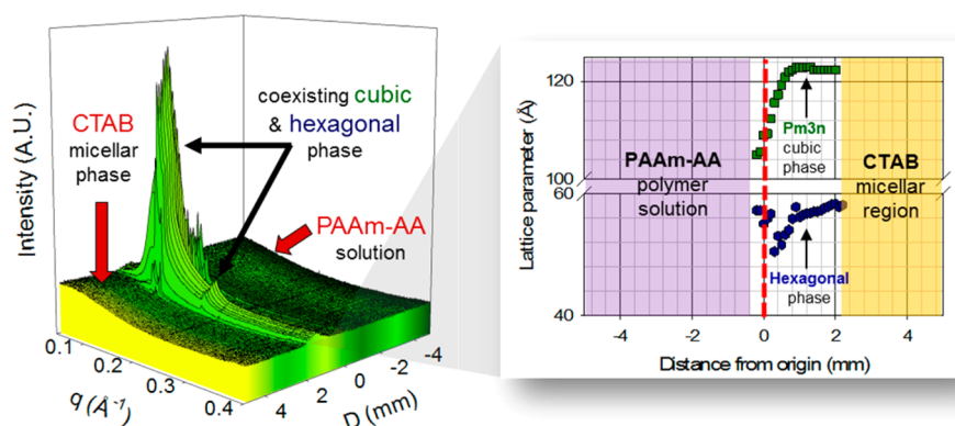
Figure 2. SAXS scattering profiles as a function of distance from origin, D , obtained during a spatial line scan across a system comprised of 2.5 wt % CTAB (top) and 1 wt % PAAm-AA solution (bottom). Coexisting cubic and hexagonal phase was shown to predominantly grow toward the bulk CTAB region after 1 week from initial contact between the two solutions (0 mm). This behavior and the differences in the lattice parameter of the Pm3n cubic (squares) and hexagonal (circles) phases formed at the interface is mapped and highlighted on the right. See the Supporting Information for q vs intensity profiles at three pertinent representative D values (Figure S2).
