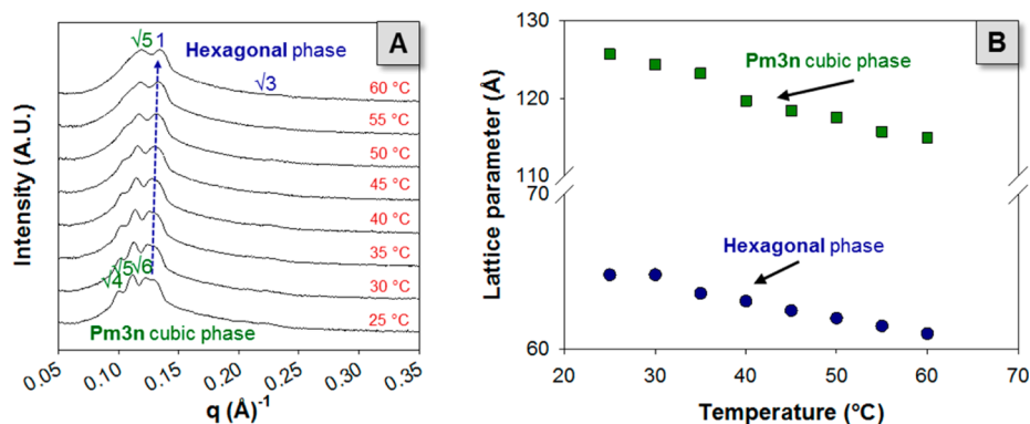
Figure 3. Influence of temperature on the equilibrium phase behavior of coexisting cubic and hexagonal existing in a mixture comprised of 2.5 wt % CTAB and 1 wt % PAAm-AA. (A) SAXS scattering profiles obtained for the system when heated from 25 to 60 °C at 5 °C increments. (B) Changes in the lattice parameter (size) of coexisting Pm3n cubic (squares) and hexagonal (circles) phases in response to heating.
