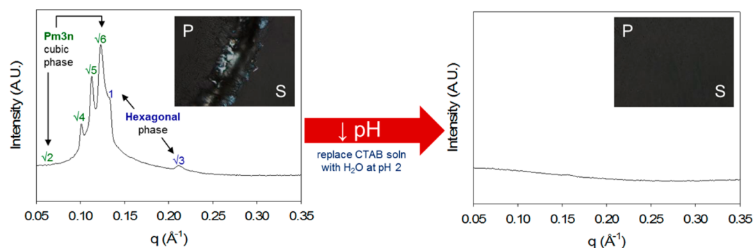
Figure 4. Effect of solution pH on the structural integrity of mesophase(s) formed at the CTAB–PAAm–AA interface. SAXS scattering profile shows the loss of coexisting cubic and hexagonal phases (left) after flushing the system with acidic solution (right). Insets: CPLM images.
