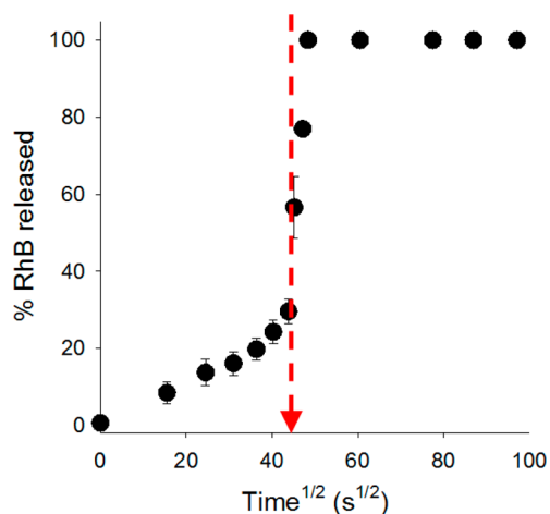
Figure 5. Cumulative % release profile of Rhodamine B (RhB) from structured CTAB–PAAm–AA capsules at ca. 37 °C ( n = 3 ). The dashed arrow indicates when the surfactant solution (pH 7) was replaced with Milli-Q water at pH 2; the point at which burst release of the dye was observed because of loss of structure at acidic conditions.
